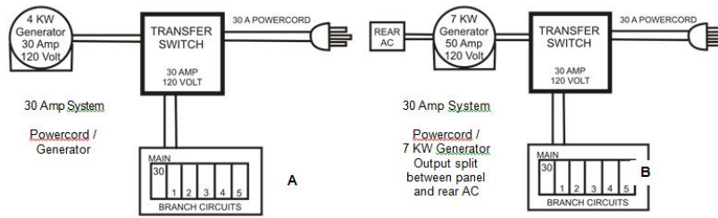
Diagram 1 – Typical Generator Powercord Connection
