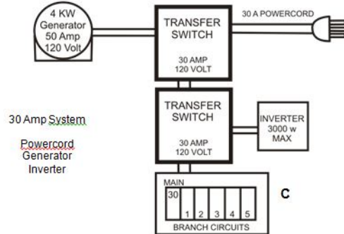
Diagram 2 – Typical Generator inverter / Alternate Source Connection
