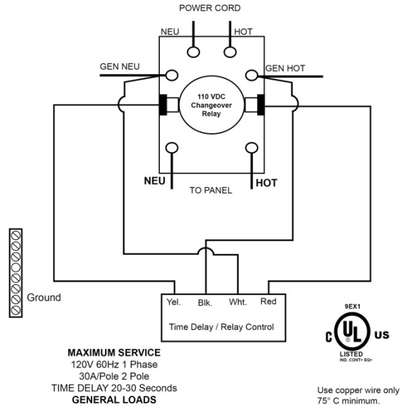
Diagram 1 – Typical Generator Powercord Connection
